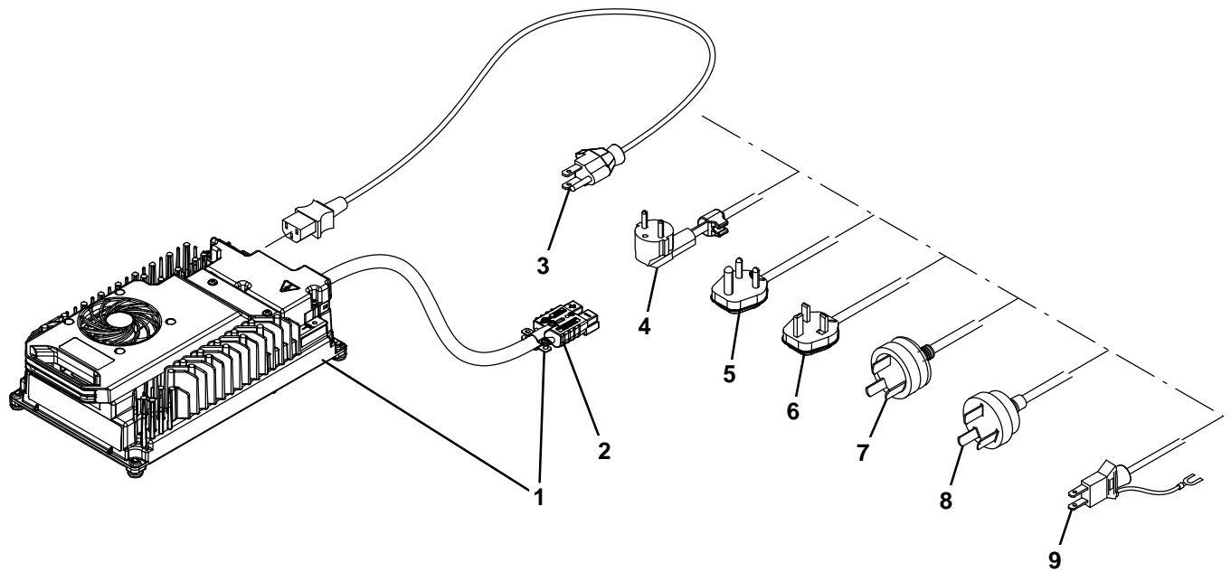
Fig. 3 – Battery Charger
