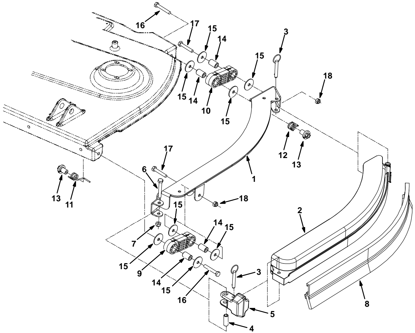
Fig. 13 – Disk Scrub Head Side Squeegee Group, Left
